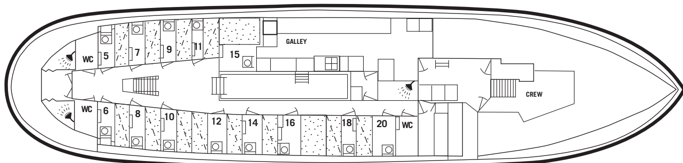
MAIN DECK
