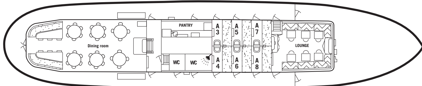
MAIN DECK
